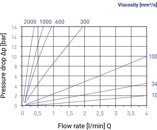
Typical pressure drop VZ0.04AL
