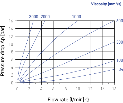
Typical pressure drop VZ0.2AL
