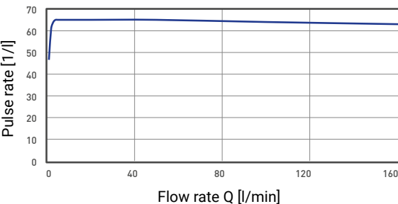
Characteristic curve
